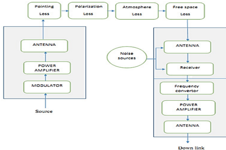
Fig. 1. Main Block Diagram of Satellite Communication System
