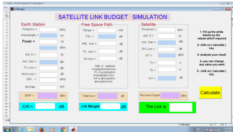
Fig. 2. shows the final active screen of satellite link budget simulation
