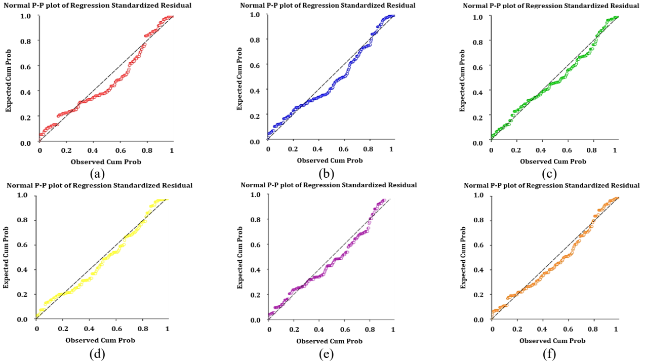
Fig. 7 Standardized residuals P-P plot for regression analysis (a) Y , (b) c , (c) \phi , (d) \alpha , (e) H and (f) r_u .
