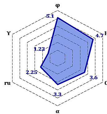
Fig. 18 Multi-factor sensitivity score of input parameters
