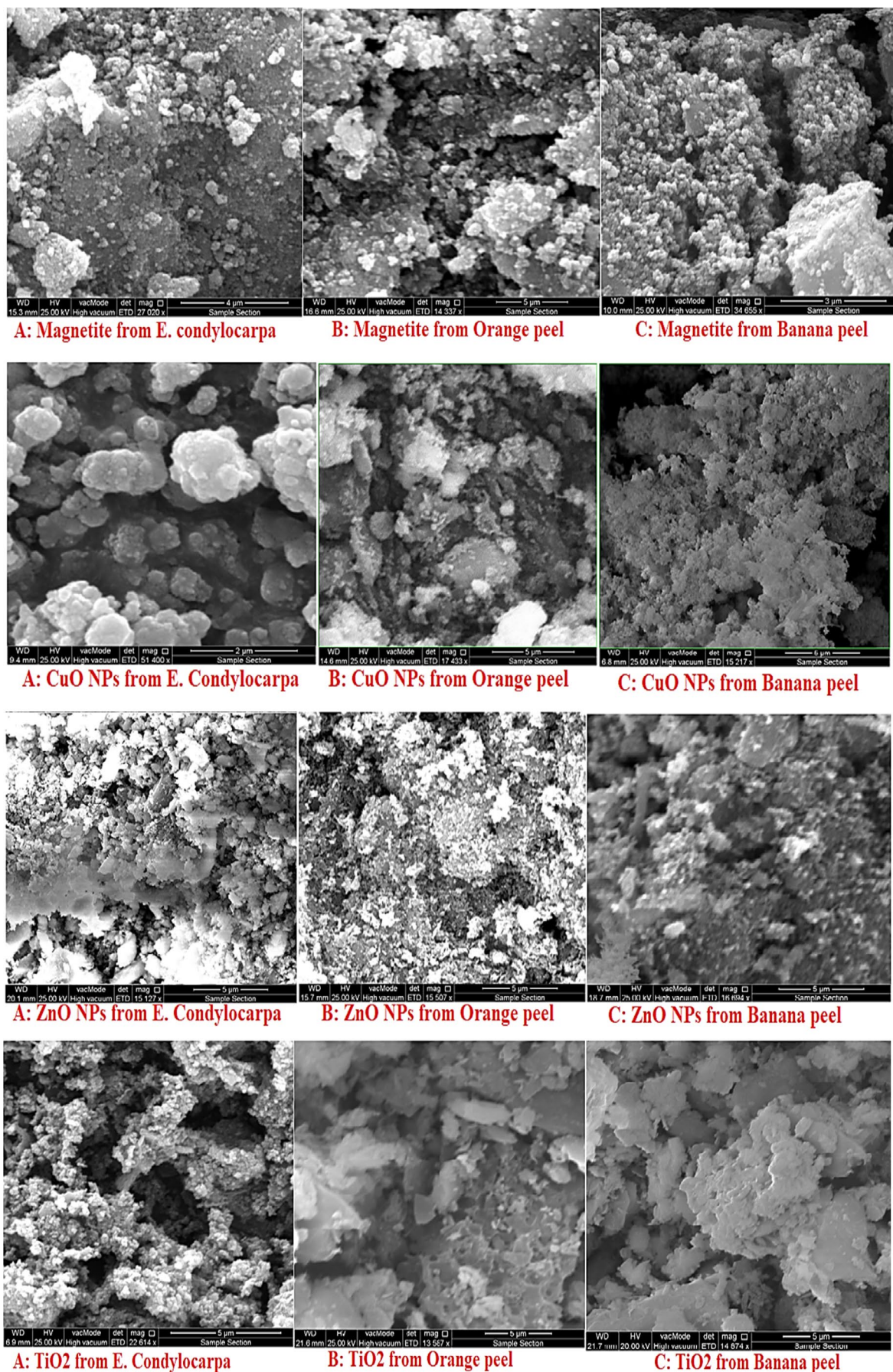
FIGURE 5 SEM analysis of various metal oxide nanoparticles using the antioxidant and reducing ability of different green sources including plant and fruit wastes
