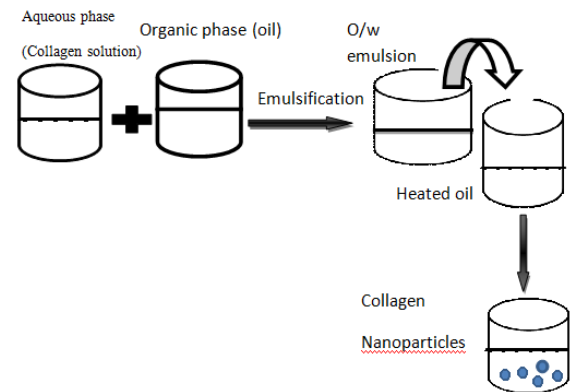
Fig.2. Emulsification method for nanoparticles manufacturing
