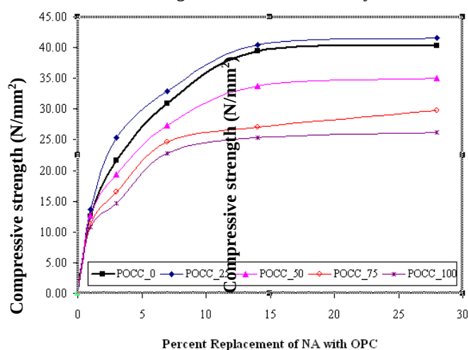
Figure 1 Compressive strength versus % replacements within 28 days
