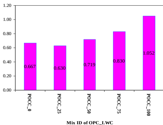
Fig 3 Results for water absorption test of OPC_LWC
