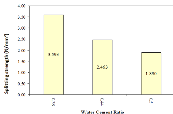
Fig. 8 Effect of water cement ratio on 28 splitting strength of POLWC
