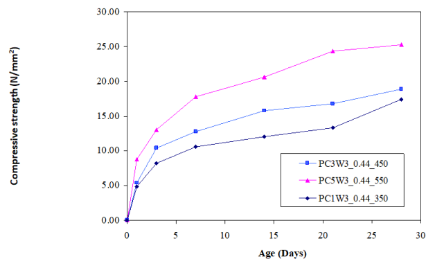
Fig 9 Effect of cement content on compressive strength of POLWC at different curing age
