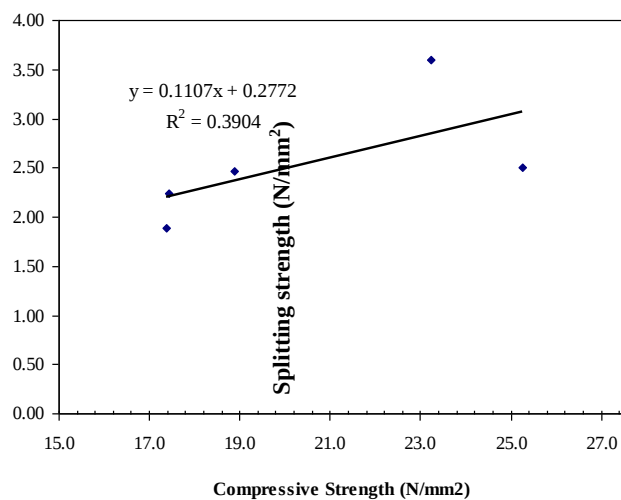
Fig. 14 Relationships between 28 days compressive strength and splitting strength of POLWC
