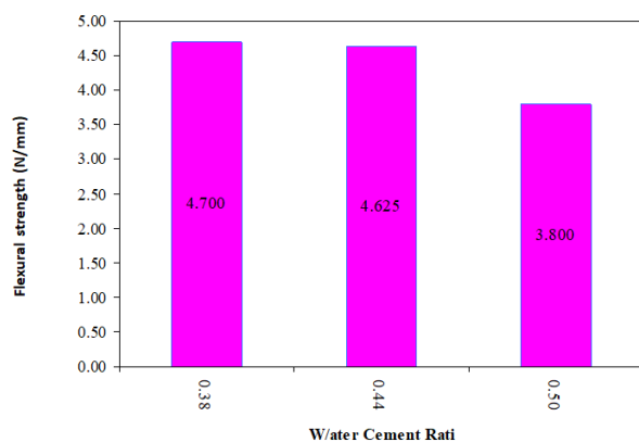
Fig 7 Effect of water cement ratio on 28 days flexural strength of POLWC
