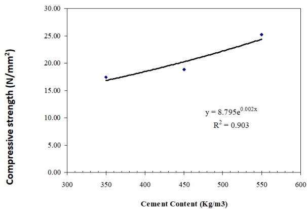
Fig 11 Relationships between Cement Content and 28 Days Compressive Strength of POLWC
