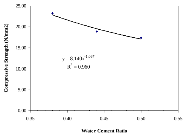
Fig. 6 Relationships between water cement ratio and 28 days compressive strength of POLWC
