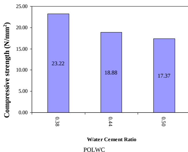
Fig 5 Effect of water cement ratio on 28 days compressive strength of
