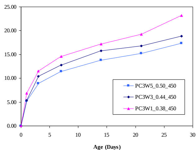
Fig 4 Effect of water cement ratio on compressive strength of POLWC
