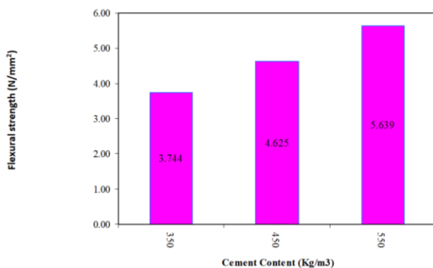
Fig 12 Effect of Cement Content on 28 Flexural Strength of POLWC
