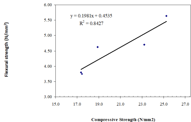
Fig 13 Relationships between 28 days compressive strength and flexural strength of POLWC
