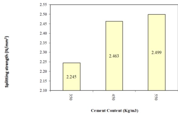
Fig 13 Effect of cement content on 28 splitting strength of POLWC
