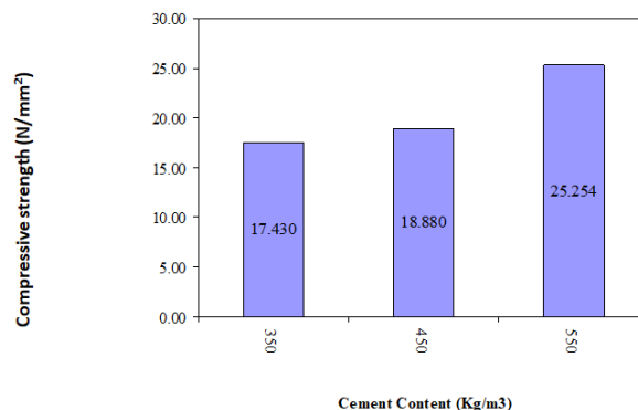
Fig 10 Effect of cement content on 28 days compressive strength of POLWC
