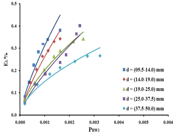
Fig. 6. The discharge-energy dissipation dimensionless relation for S.R.W.J.
