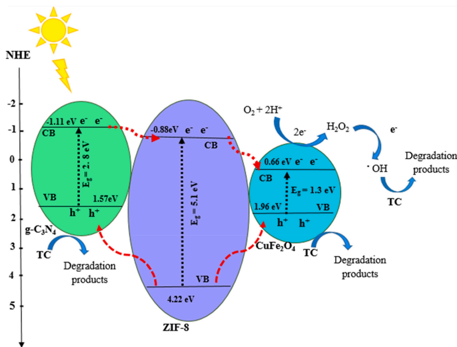
Fig. 13. Proposed photocatalytic mechanism of TC over the ZIF-8/g-C 3 N 4 /CuFe 2 O 4 .
