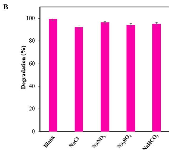
Fig. 9. Effect of humic acid (A), and ions (B) on the photodegradation efficiency of TC by ZIF-8/g-C 3 N 4 /CuFe 2 O 4 ( C_{\text{Photocatalyst}} = 0.75 g/L, C_{\text{TC}} = 15 ppm, and pH=5).
