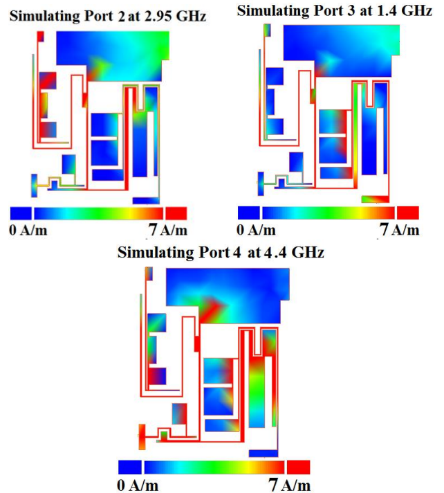
FIGURE 4. Current density distribution of the designed triplexer.
