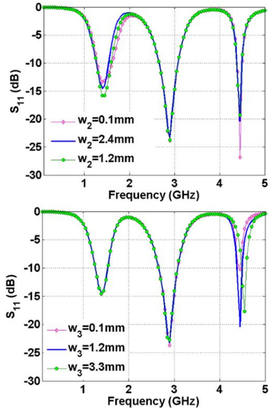
FIGURE 6. S_{11} as functions of the significant physical dimensions.
