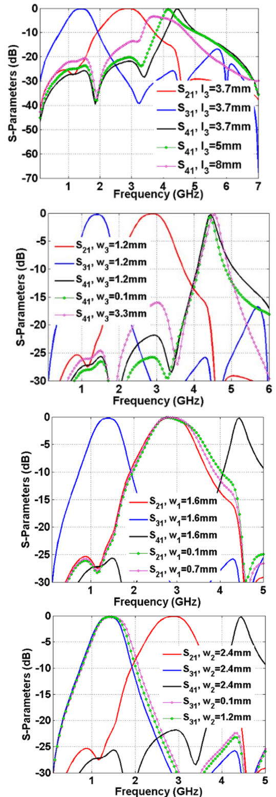
FIGURE 5. Frequency responses as functions of the significant physical dimensions.
