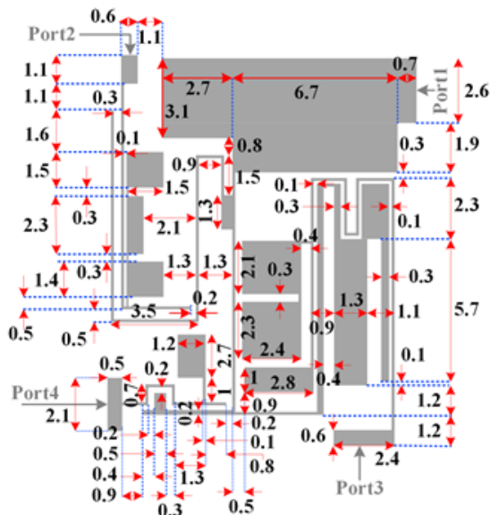
FIGURE 2. Proposed BPFs: layouts and frequency responses (Unit: mm and all the thinnest lines have widths of 0.1 mm).
